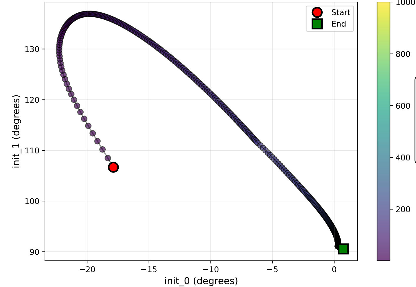
Optimization Trajectory
